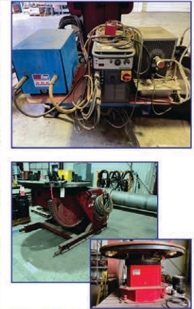
Clad Unit #5: Vanguard LHZ34 Cladding Machine with Arc Specialties Hot One Solid State Hotwire Power Supply Esab MTS-3500i MIG Welder, Note: (2) rotary tables avail.
